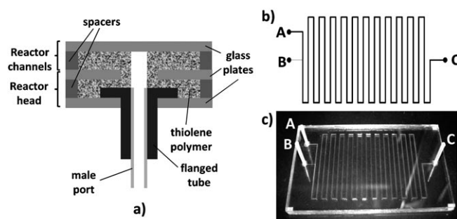
Figure 1. a) Female port design in the MR head that serves as a base for the microchannels network; b) mask used for the reactor photo-patterning; c) glass-thiolene reactor with three female ports: substrate inlet (A), oxygen inlet (B), product outlet (C).
