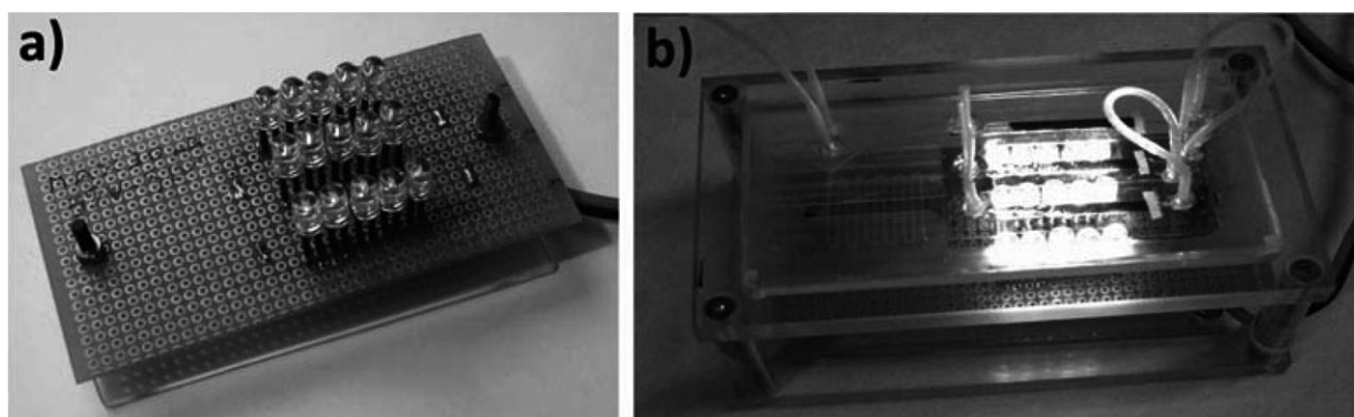
Figure 6. a) LED 5 \times 3 array; b) MR of Figure 2 with LED source turned on.
