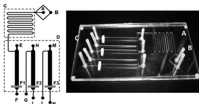
Figure 2. Microfluidic path for the photochemical MR. Oxygen inlet (A), substrate solution inlet (B), oxygenation zone (C), micro-chamber zone (D), photocatalyst feed ports (E, H, M), outlet/connection ports (F, G, I, L, N), paper filter restraints (F1, F2, F3).
