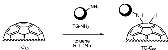
Figure 4. Supporting [60]fullerene on Tentagel® beads.
