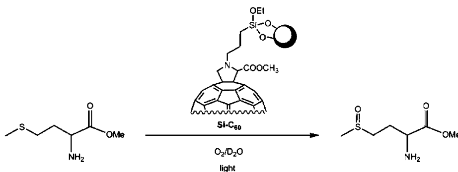
Figure 5. Photooxidation of methionine to methionine sulfoxide.
